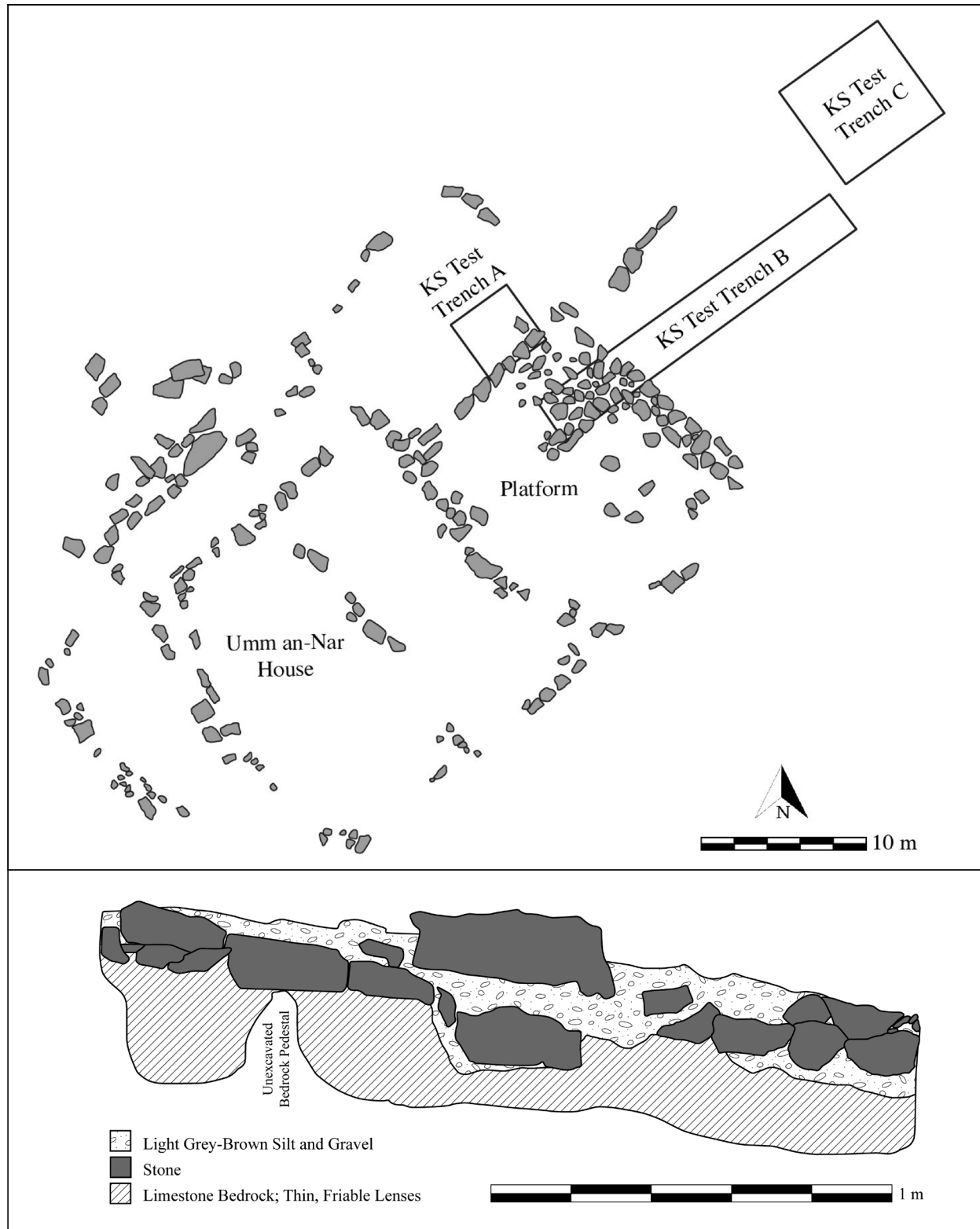
Figure 8: Plan of Khutm east complex indicating locations of the probable Umm an-Nar house and platform, and Test Trenches A–C (top; plan by Jennifer Swerida); KS Test Trench A southeast profile (bottom; profile by Robert Bryant).
