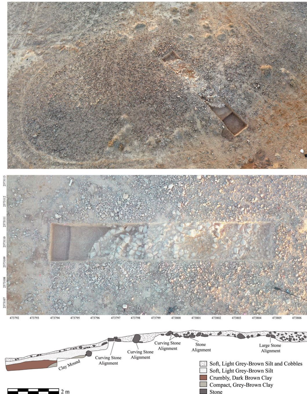
Figure 5: Oblique image of Operation A from the west the results of the 2x11m trench (top); Overhead of Operation A excavation (middle; image by Robert Bryant); South profile of the Operation A excavation (bottom; profile by Jennifer Swerida).
